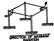
Rhombic antenna.
